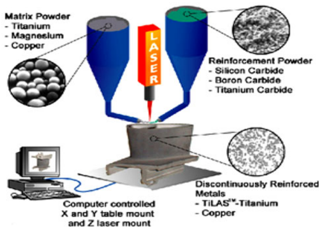
Fig. 1 Schematic view of laser forming
