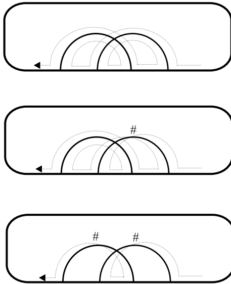
Figure 9 Factoring out two-humped camels; notice that a chord being slid over the camel will follow the same path whether it is marked or unmarked, and that its marking after being slid over the camel will be the same as before (although it may change during the process)
