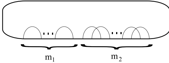
Figure 3 Example of an (m_1, m_2) -caravan
