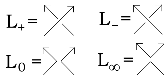
Figure 4 Diagrams of the skein relation
