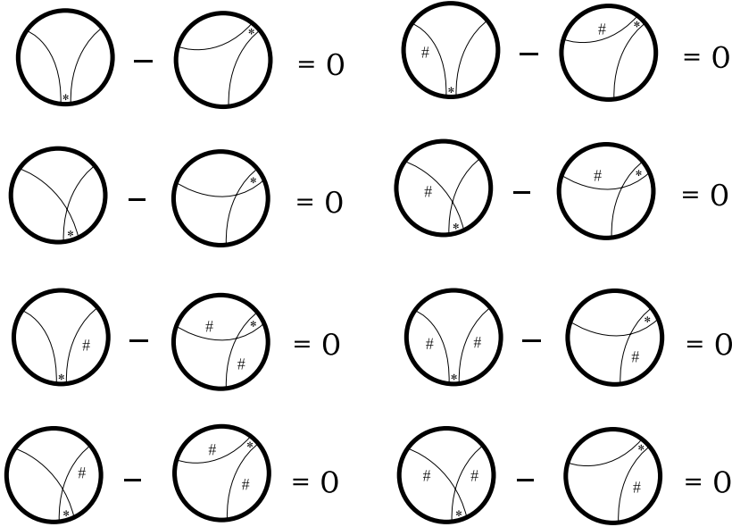
Figure 7 2-term relations on marked chord diagrams
