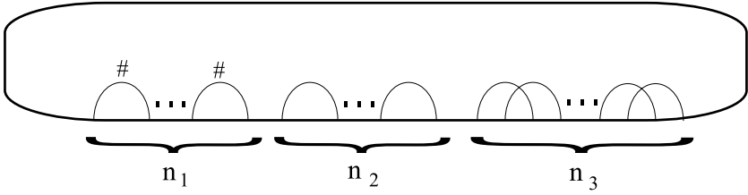
Figure 8 A marked (n_1, n_2, n_3) -caravan
