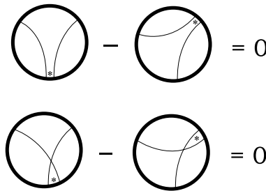
Figure 2 The 2-term relations
