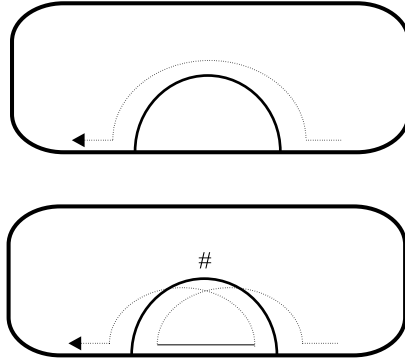
Figure 10 Factoring out one-humped camels; notice that a chord being slid over the camel will follow the same path whether it is marked or unmarked, and that its marking after being slid over the camel will be the same as before (although it may change during the process)
