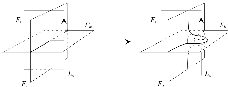
Figure 5: Second finger move
