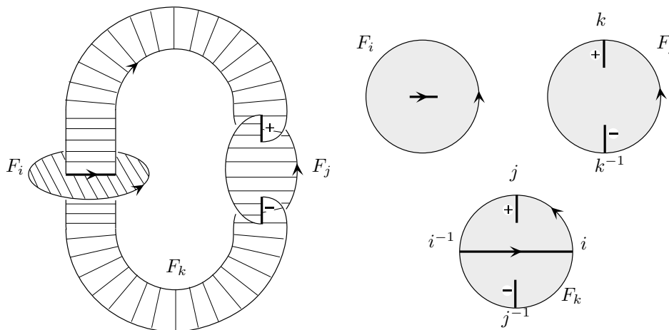
Figure 2: Computation of m_{ijk}
