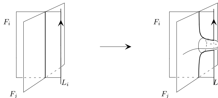
Figure 4: First finger move
