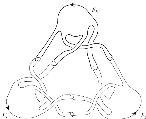
Figure 3: Disentangled surfaces
