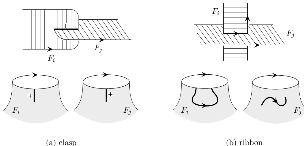
Figure 1: Intersections of Seifert surfaces
