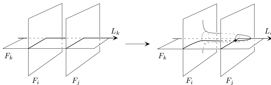
Figure 6: Third finger move
