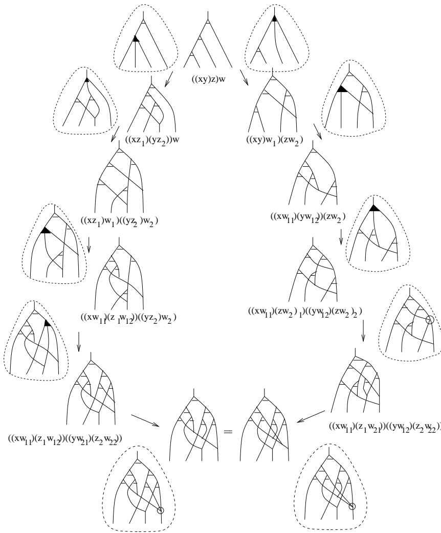
Figure 28: First 3-differential, d^{3,1}
