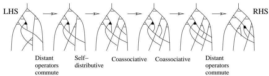
Figure 40: The term 12
