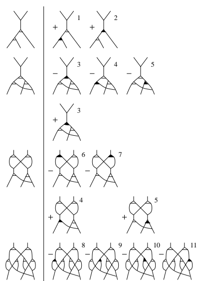
Figure 34: d^{3,2}D_2(\eta_1, 0) , LHS
