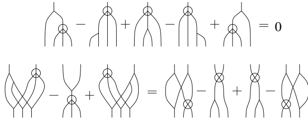
Figure 19: Hochschild 3-cocycle conditions
