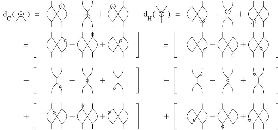
Figure 18: Hochschild 2-differentials
