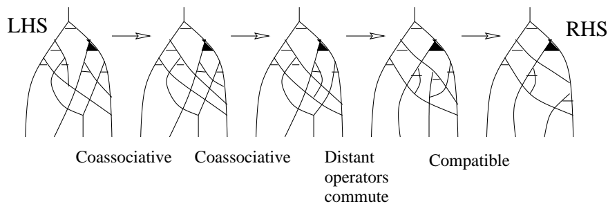
Figure 41: The term 13
