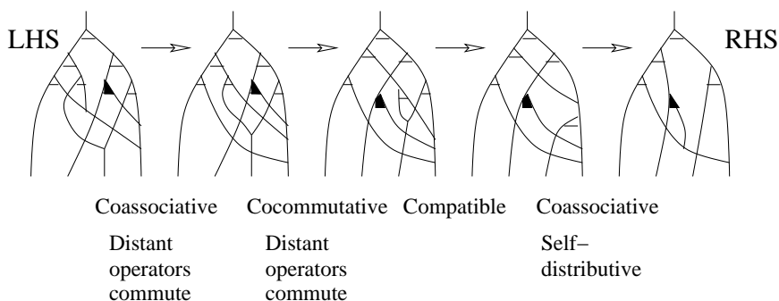
Figure 42: The term 14
