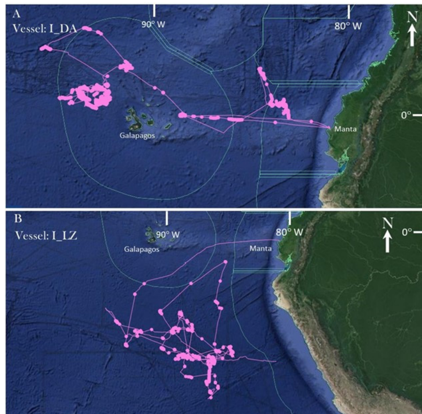
Figure 2. Fishing route (pink line) of industrial fishing vessels (A) I_DA and (B) I_LZ based on AIS information. Fishing duration was 35 and 76 days, respectively. Green line indicates Economic Exclusive Zones of 200 nautical miles from shore. Imagery adapted from GlobalFishingWatch.org.
