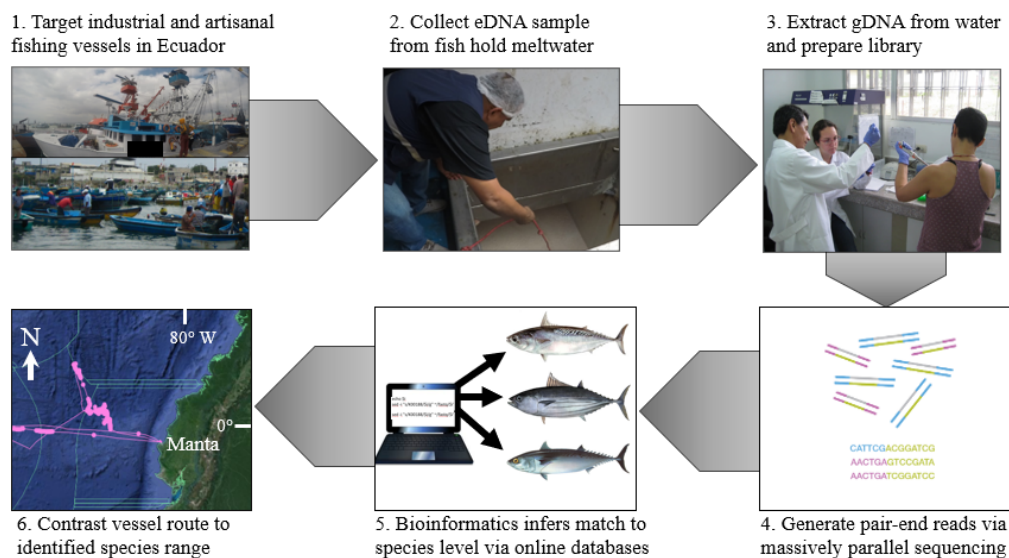
Figure 1. Schematic overview of experimental design using eDNA metabarcoding to characterize fish catch from industrial and artisanal fishing vessels in Ecuador.
